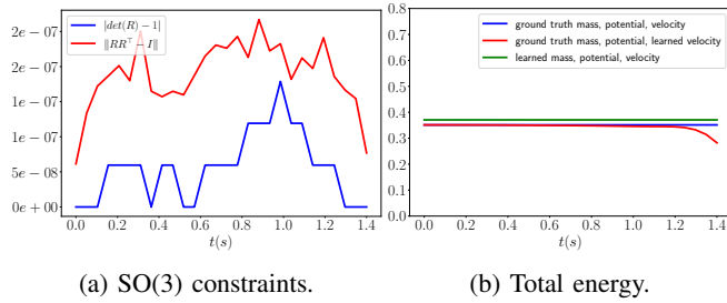
Fig. 4: SO(3) constraints and total energy along a trajectory rollout with zero control input from the learned rigid body model.
